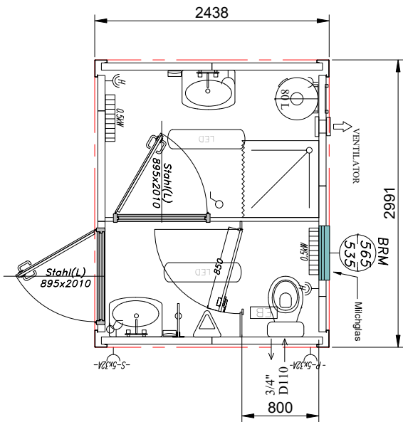
Containerplan MS 10
