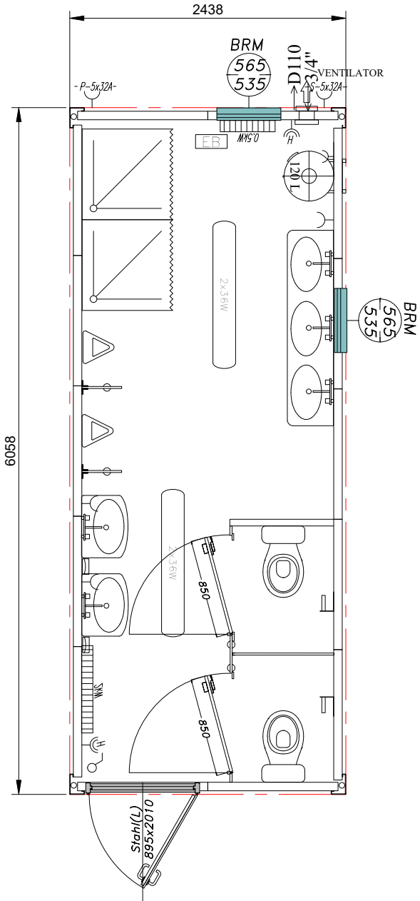
Containerplan MS 20
