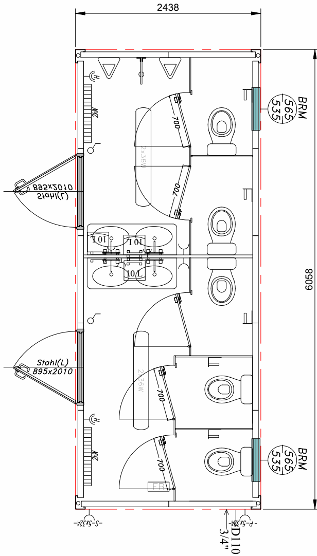
Containerplan MW 23
