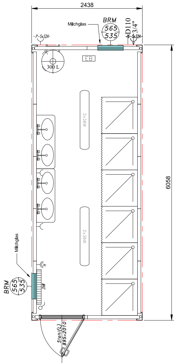
Containerplan MZ 20
